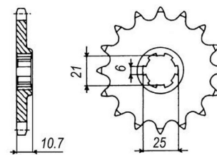
Chain 630
